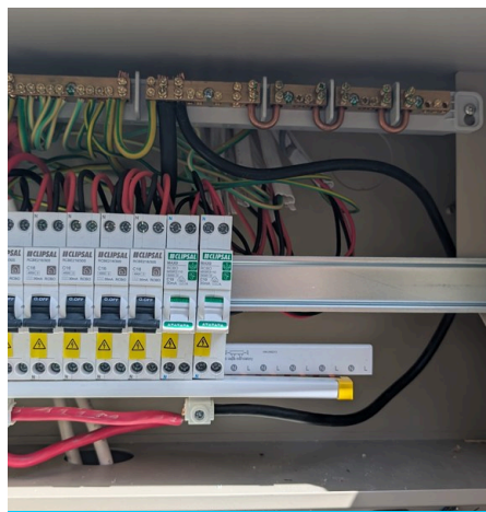
Switchboards
